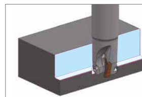
Shoulder milling
